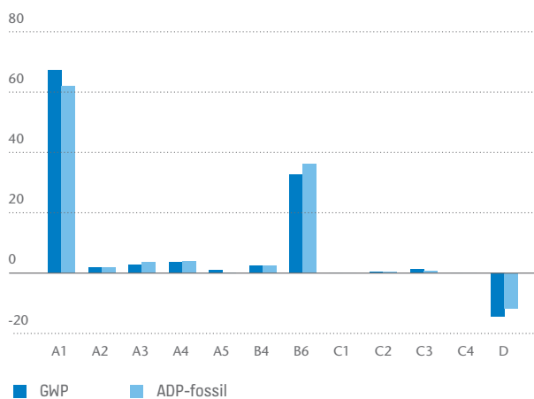
Figure 1. Results for GWP and ADP of fossil resources of KONE MonoSpace 300 elevator
